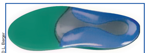
Figure 1. The thermoformed plantar orthotics with lateral reinforcements (OR) comprised a base of Transflux® resin (1 mm), identical lateral reinforcements, an Evamic® top layer (2.5 mm), Orthomic® at the rear foot (3 mm) and Viscotène® at the forefoot (2.5 mm).
